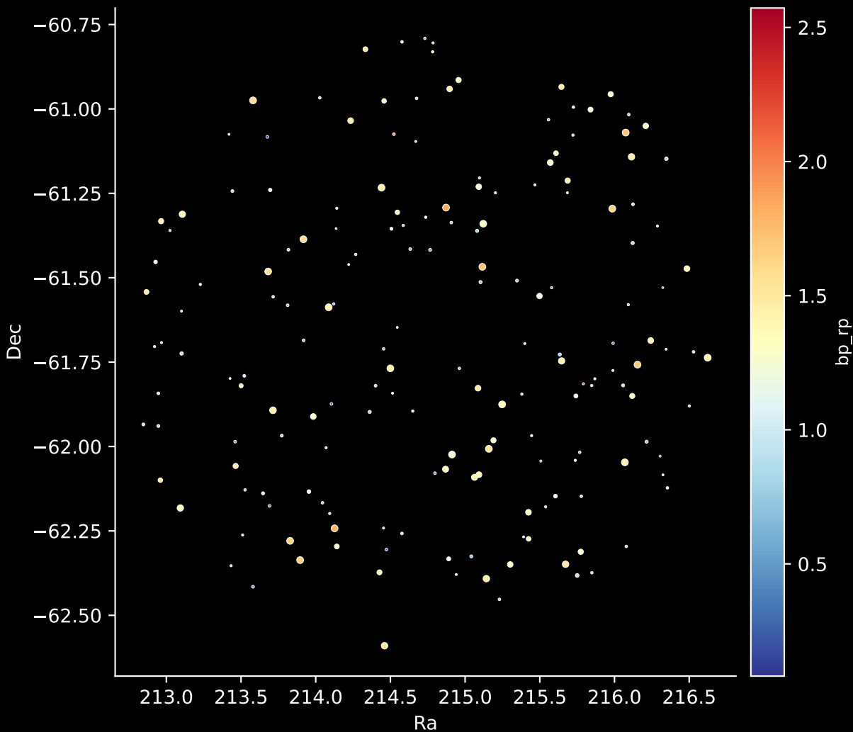
APOGEE DR17 Field: [274-18-O_TESS] Stars: 176
