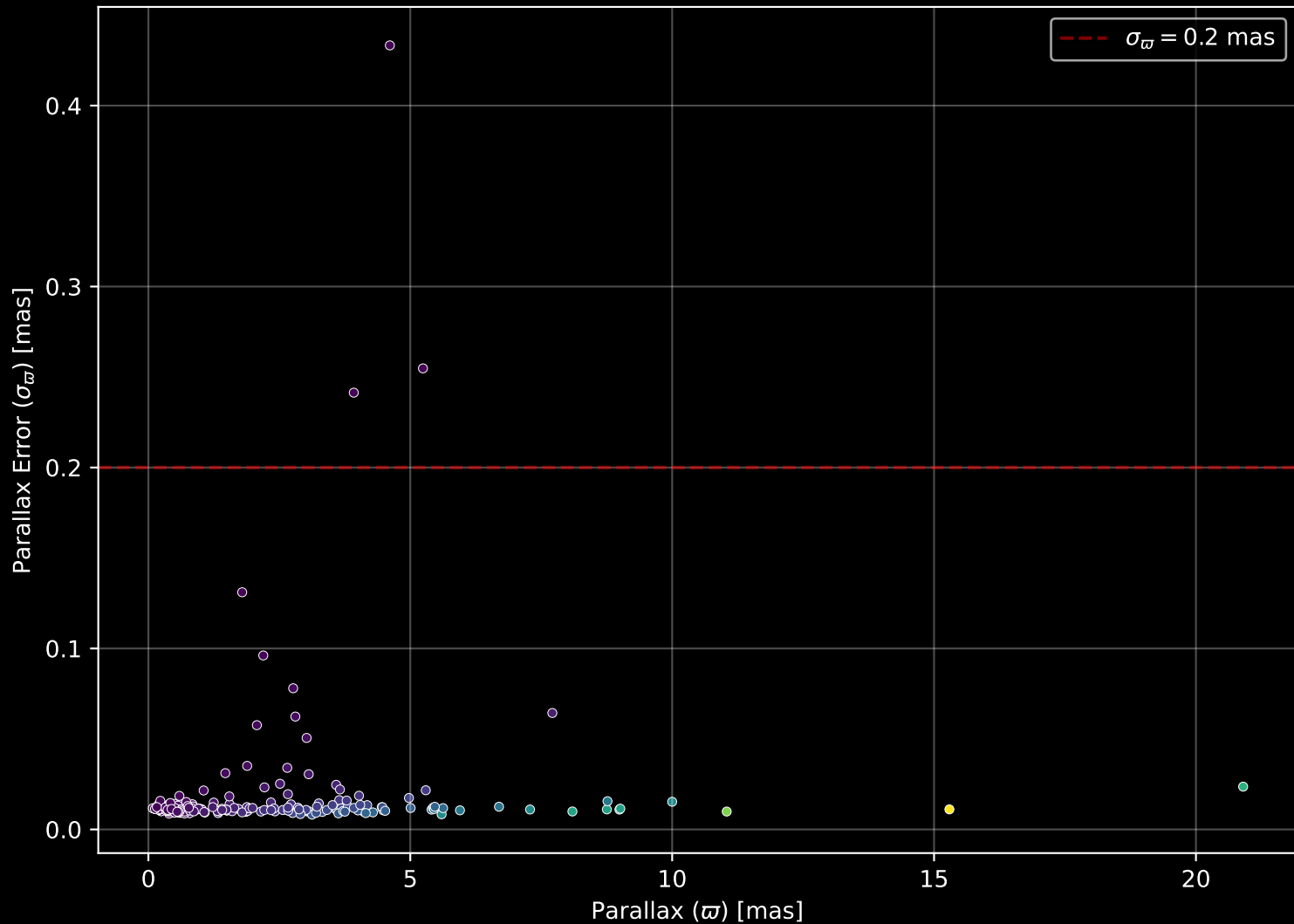
APOGEE DR17 Field: [274-18-O_TESS] Parallax Quality (n= 176)
