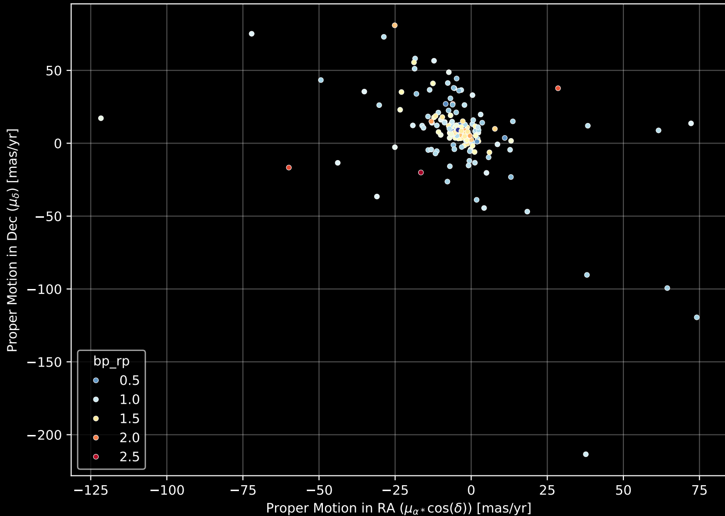
APOGEE DR17 Field: [274-18-O_TESS] Proper Motion Diagram (n= 176)
