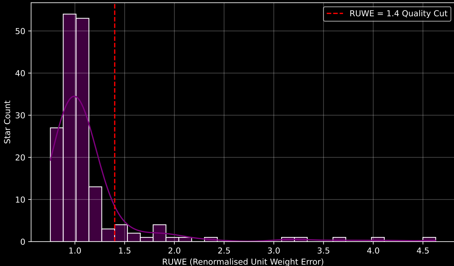
GAPOGEE DR17 Field [274-18-O_TESS] RUWE Distribution (n= 169)
