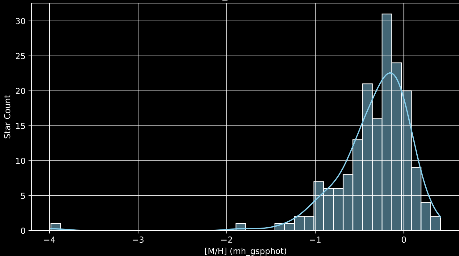
APOGEE DR17 Field: [274-18-O_TESS [M/H] (mh_gspphot) (n= 175)
