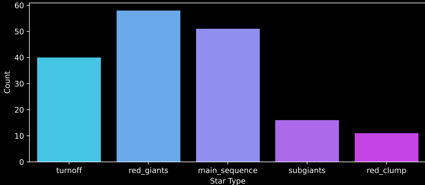
APOGEE DR17 Field: [274-18-O_TESS] Count plot of Star Type
